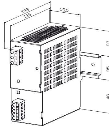
Abb. 1 Dimensions on Mounting Rail TH35 Fig. 1
