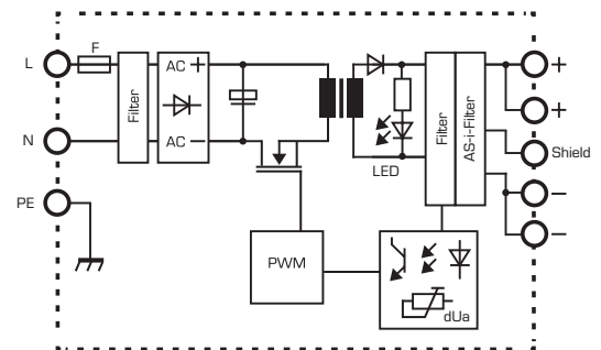
Abb. 3 Block Diagram Fig. 3
