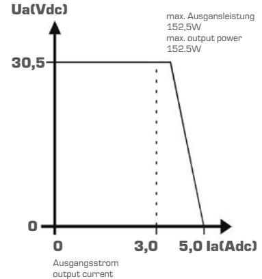
Abb. 2 Output Characteristic Fig. 2
